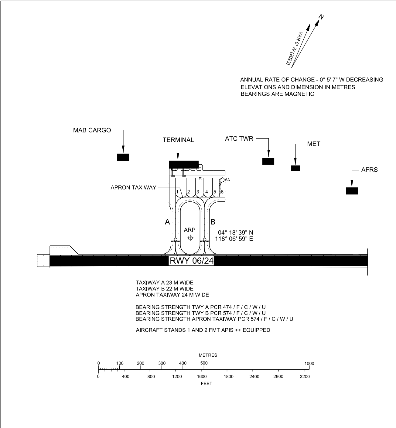
AIRCRAFT PARKING / DOCKING STAND POSITION
