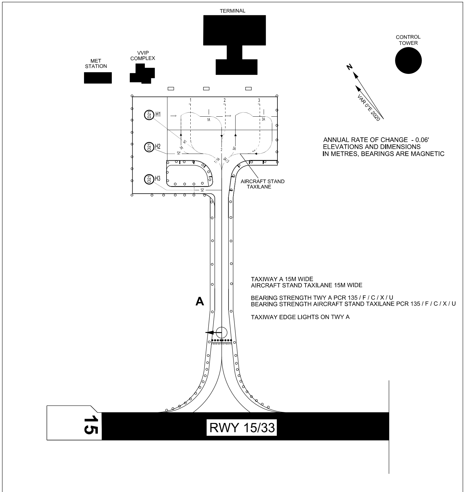
AIRCRAFT PARKING / DOCKING STAND POSITION
