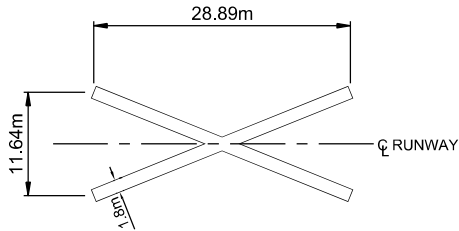
CLOSED RUNWAY 'X' MARKING
