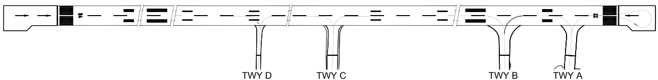
MARKING AIDS RWY 04 / 22 AND EXIT TWY
